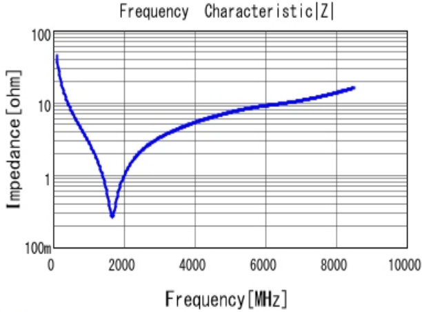
■ GRM0332C1H360JA01 |Z| DC0V, 20degC
