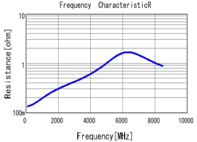
■ GRM0332C1H360JA01 R DC0V, 20degC
