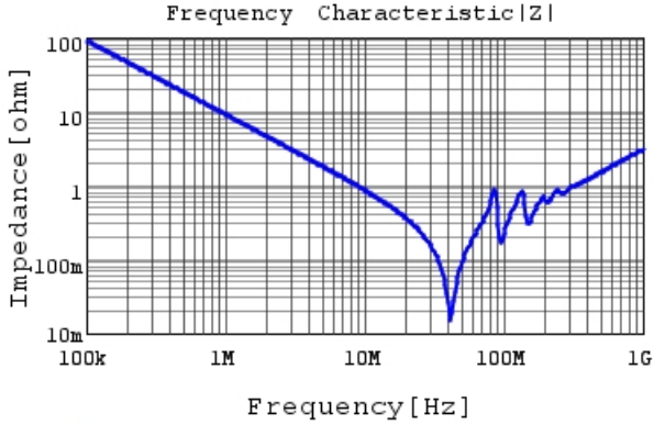
GCM32D5C2J183GX01 |Z| DC0V, 25degC
