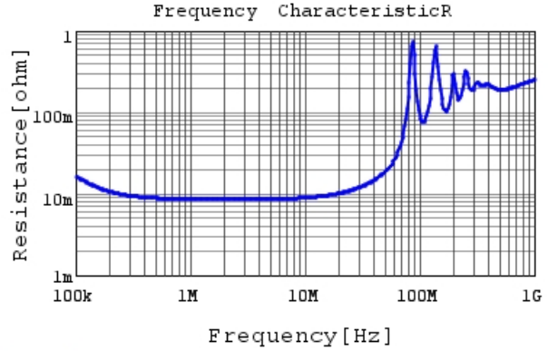
GCM32D5C2J183GX01 R DC0V, 25degC
