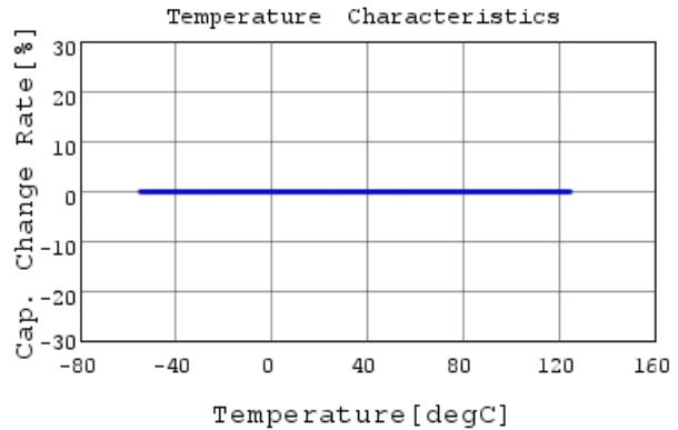
GCM32D5C2J183GX01 C-Temp. capchange, DC0V, 1
