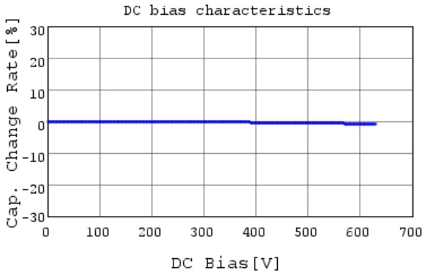
GCM32D5C2J183GX01 C-DC bias capchange, 25.0c
