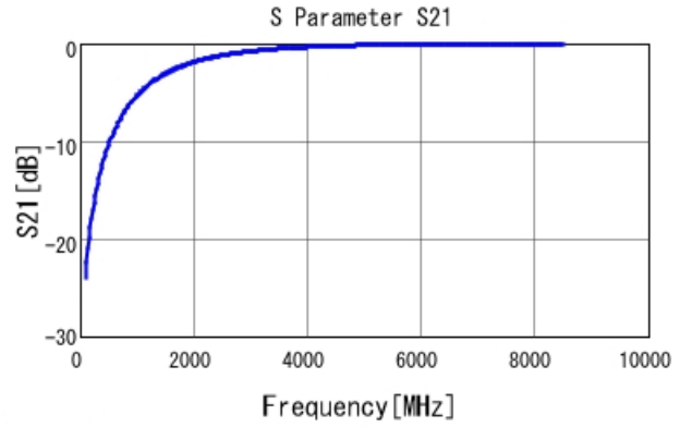
GRM1885C2A1R0CA01 S21 DCOV, 25degC
