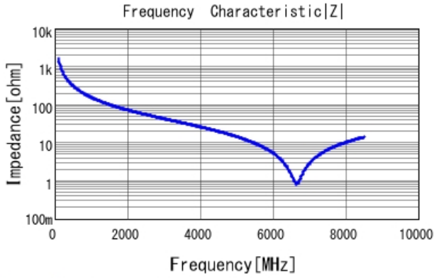
GRM1885C2A1R0CA01 |Z| DCOV, 25degC
