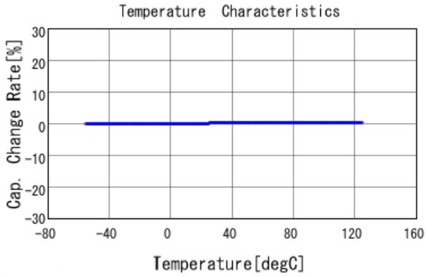
GRM1885C2A1R0CA01 C-Temp. capchange, DCOV, AC1Vrms
