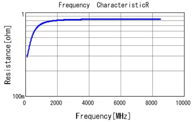
GRM1885C2A1R0CA01 R DCOV, 25degC
