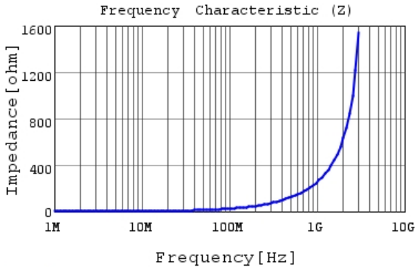
LQW15AN39NJ80 |Z|
