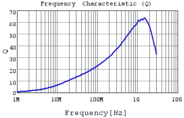
LQW15AN39NJ80 Q
