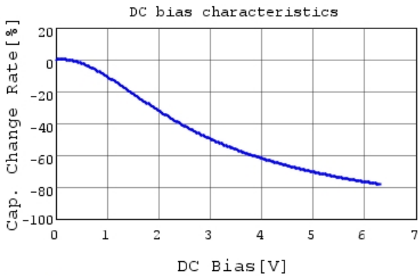
GRM033B30J224ME15 C-DC bias capchange, 20.0c
