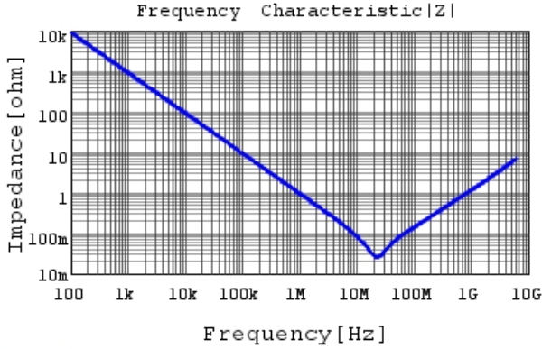
GRM033B30J224ME15 |Z| DCOV, 20degC
