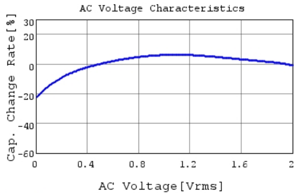
GRM033B30J224ME15 C-AC Voltage capchange, Dc
