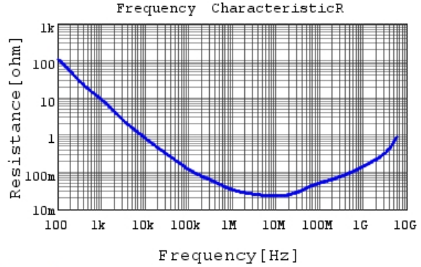
GRM033B30J224ME15 R DCOV, 20degC
