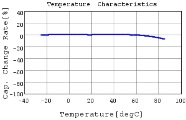
GRM033B30J224ME15 C-Temp. capchange, DC0.0V,
