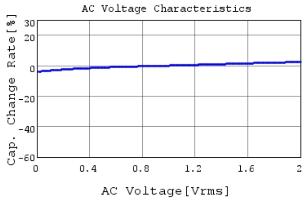
GRT155R71E103KE01 C-AC Voltage capchange, Dc
