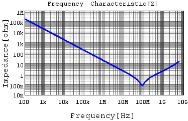
GRT155R71E103KE01 |Z| DCOV, 25degC
