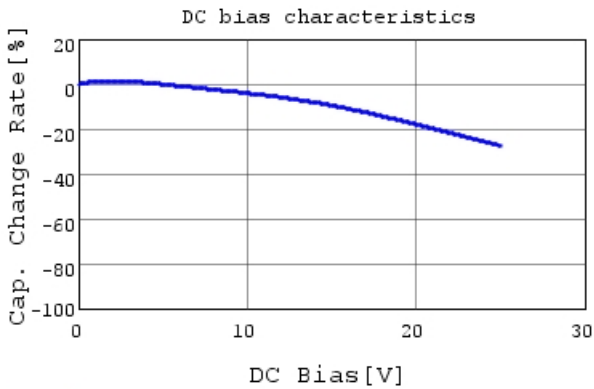
GRT155R71E103KE01 C-DC bias capchange, 25.0c
