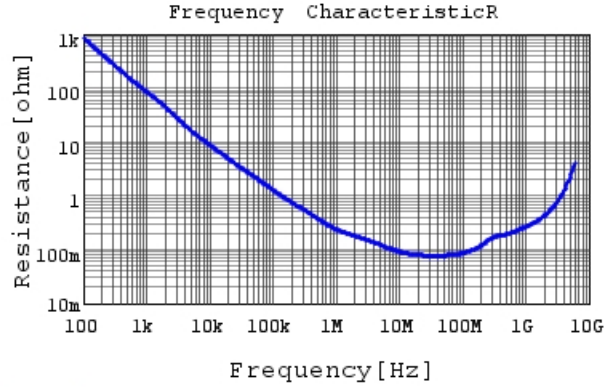
GRT155R71E103KE01 R DCOV, 25degC
