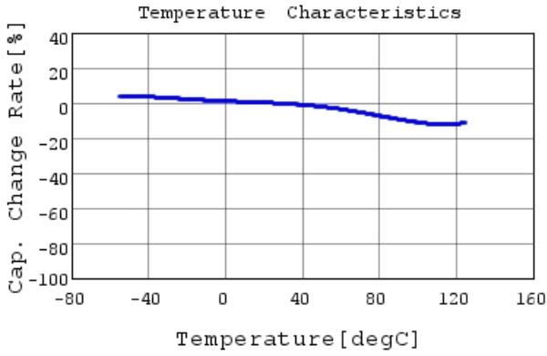
GRT155R71E103KE01 C-Temp. capchange, DC0.0V,
