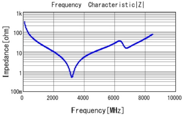
GRM1885C1H5R0BA01 |Z| DCOV, 25degC
