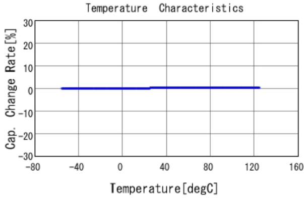
GRM1885C1H5R0BA01 C-Temp. capchange, DCOV, AC1Vrms
