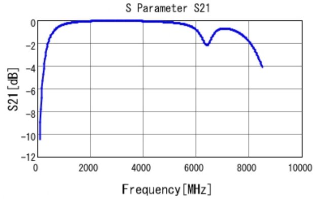
GRM1885C1H5R0BA01 S21 DCOV, 25degC
