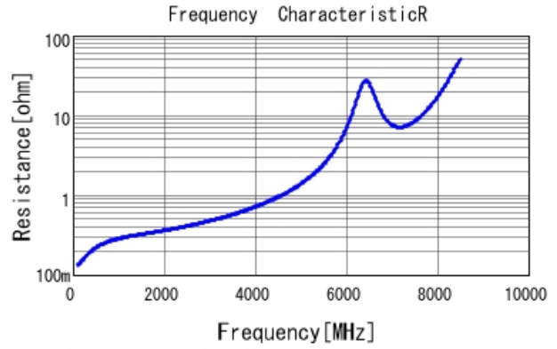
GRM1885C1H5R0BA01 R DCOV, 25degC
