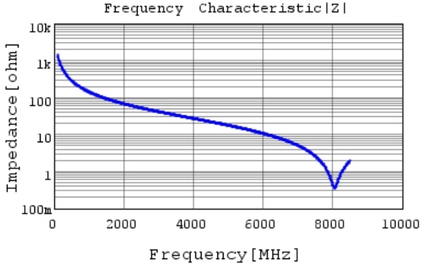
GCQ1555C1H1R1CB01 |Z| DCOV, 25degC
