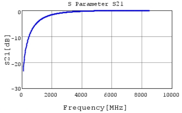
GCQ1555C1H1R1CB01 S21 DCOV, 25degC
