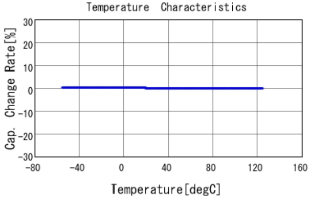
GRM1552C1H681JA01 C-Temp. capchange, DCOV, AC1Vrms
