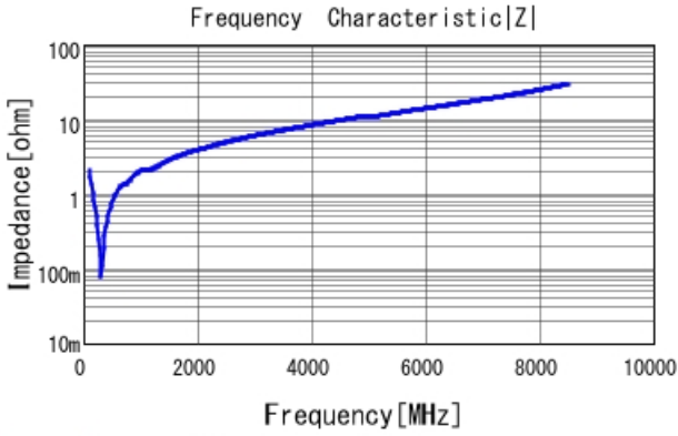
GRM1552C1H681JA01 |Z| DCOV, 20degC
