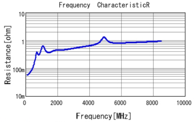
GRM1552C1H681JA01 R DCOV, 20degC
