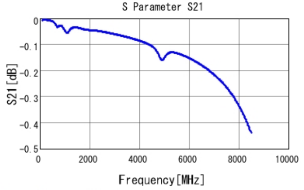
GRM1552C1H681JA01 S21 DCOV, 20degC
