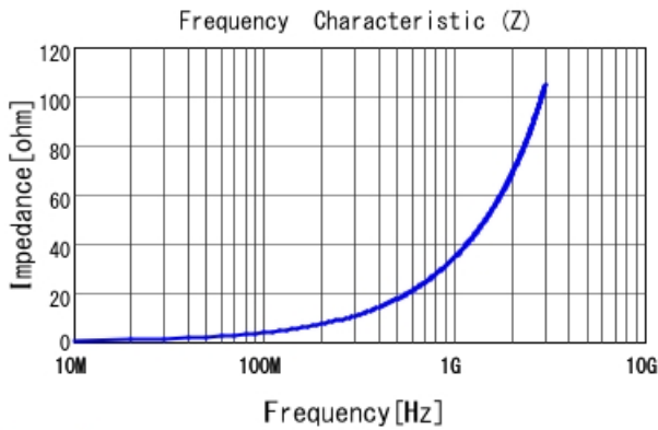
LQP02TQ5N6H02 |Z|
