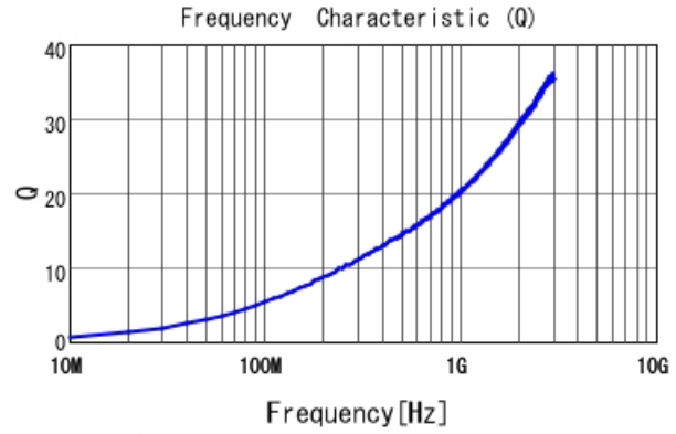
LQP02TQ5N6H02 Q
