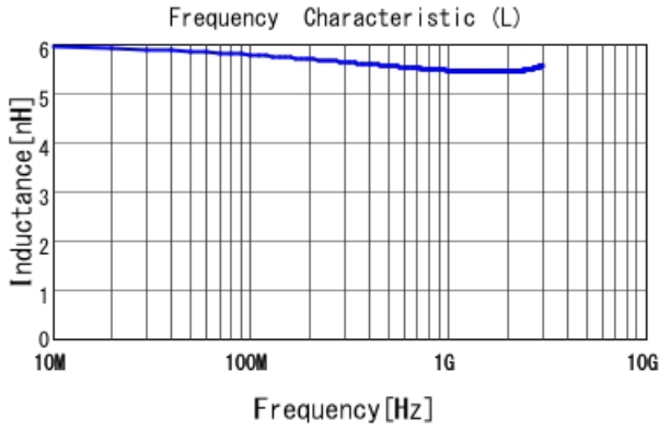
LQP02TQ5N6H02 L
