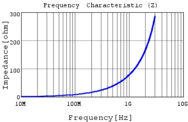
LQW03AW12NJ00 |Z|
