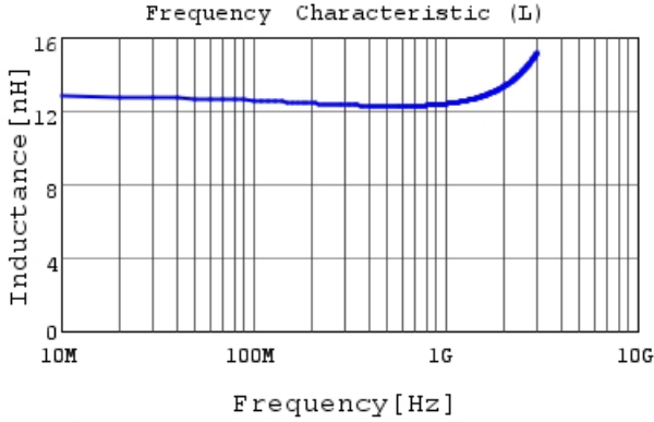
LQW03AW12NJ00 L
