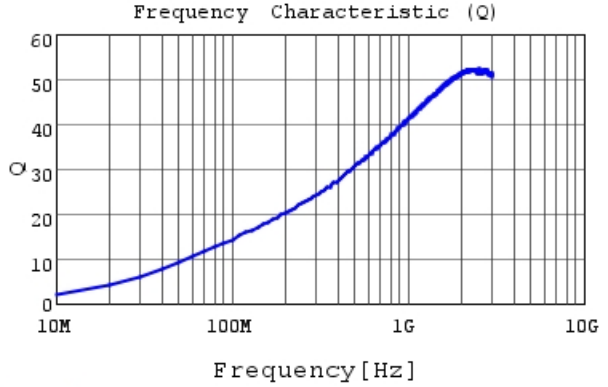
LQW03AW12NJ00 Q
