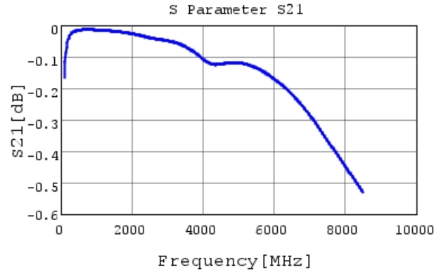
GRM0332C2A820JA01 S21 DCOV, 20degC
