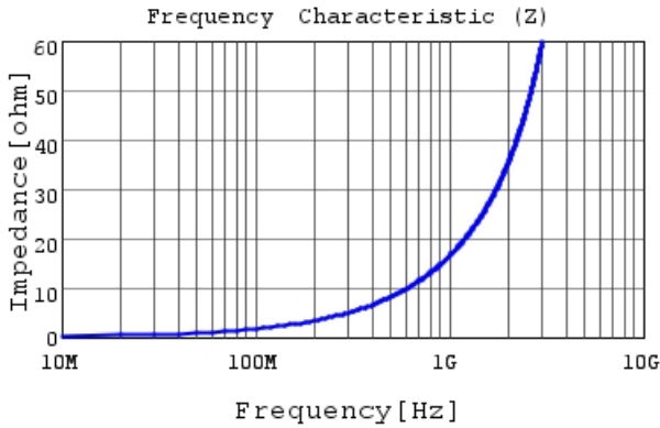
LQG15HN2N7B02 |Z|
