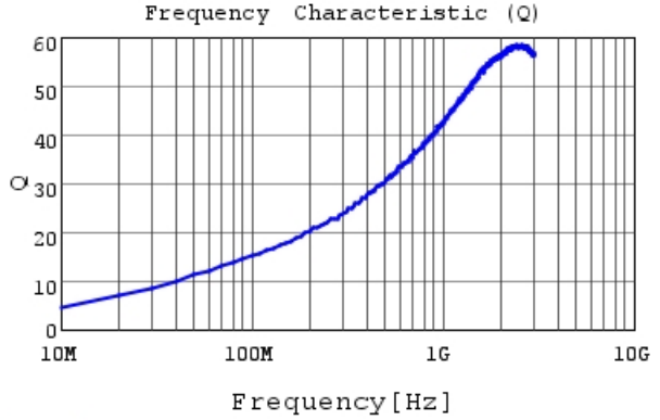
LQG15HN2N7B02 Q
