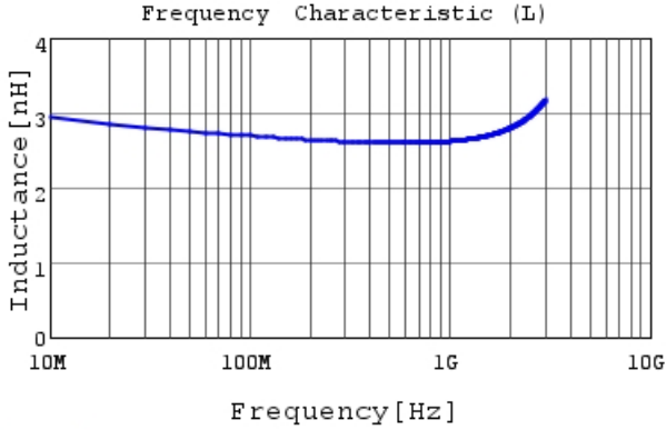
LQG15HN2N7B02 L
