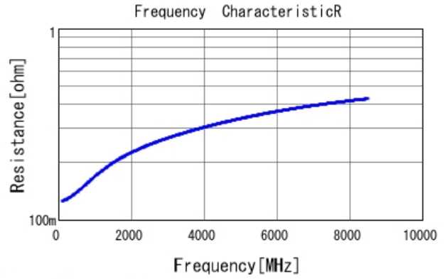
GRM0225C1E100JA03 R DCOV, 25degC
