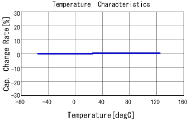
GRM0225C1E100JA03 C-Temp. capchange, DCOV, AC1Vrms
