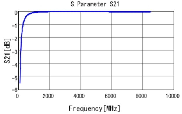
GRM0225C1E100JA03 S21 DCOV, 25degC
