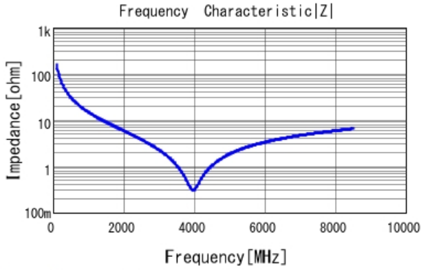
GRM0225C1E100JA03 |Z| DCOV, 25degC
