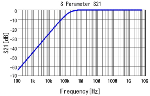
■ GRM033B31E103MA12 S21 DCOV, 20degC
