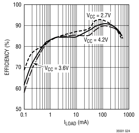
Buck Regulator Efficiency vs Output Current
