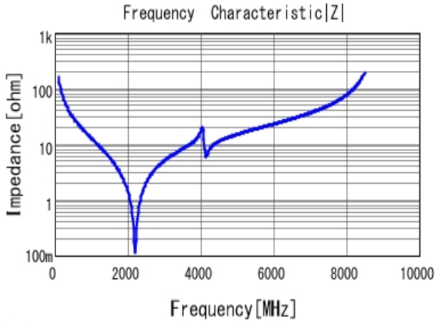
■ GQM1885C1H100GB01 |Z| DCOV, 25degC
