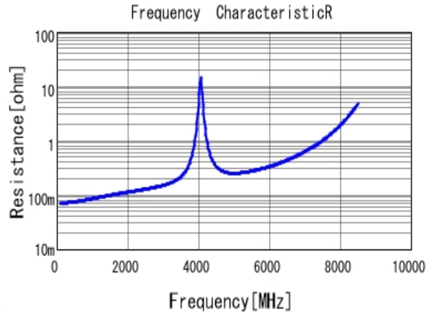
■ GQM1885C1H100GB01 R DCOV, 25degC
