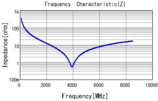
GRM1555C1E4R7CA01 |Z| DCOV, 25degC
