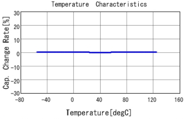
GRM1555C1E4R7CA01 C-Temp. capchange, DCOV, AC1Vrms
