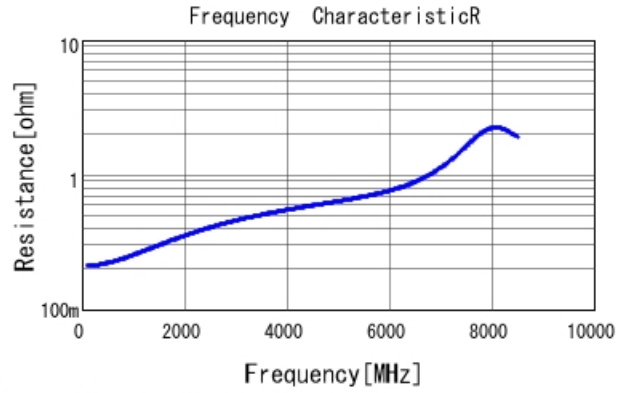
GRM1555C1E4R7CA01 R DCOV, 25degC
