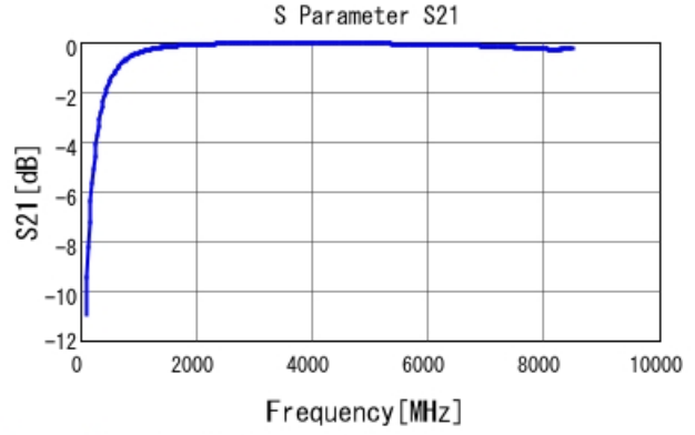
GRM1555C1E4R7CA01 S21 DCOV, 25degC
