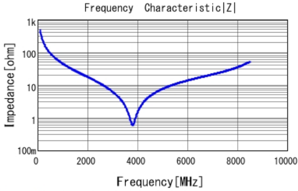
GRM1885C2A3R3CA01 |Z| DCOV, 25degC
