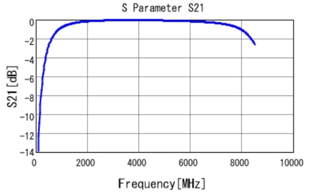
GRM1885C2A3R3CA01 S21 DCOV, 25degC
