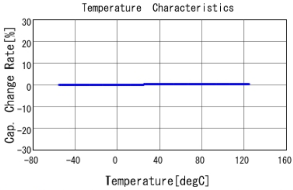
GRM1885C2A3R3CA01 C-Temp. capchange, DCOV, AC1Vrms
