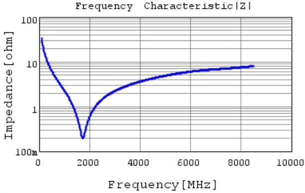
GRM0225C1E470GA02 |Z| DC0V, 25degC
