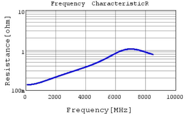
GRM0225C1E470GA02 R DC0V, 25degC
