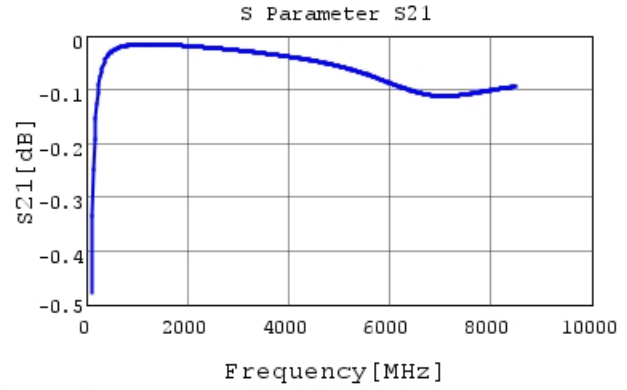
GRM0225C1E470GA02 S21 DCOV, 25degC
