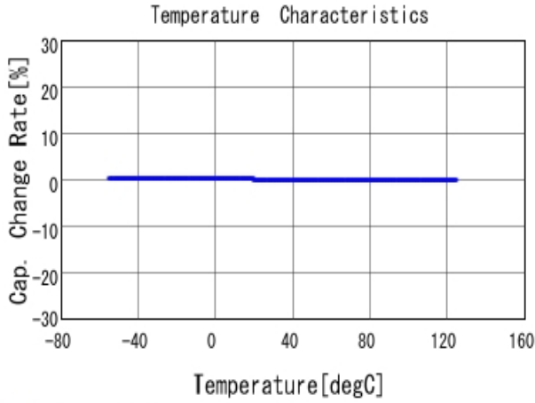
■ GRM0332C1H180GA01 C-Temp. capchange, DCOV, AC1Vrms
