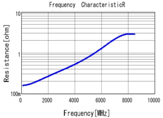
■ GRM0332C1H180GA01 R DCOV, 20degC
