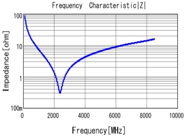
■ GRM0332C1H180GA01 |Z| DCOV, 20degC
