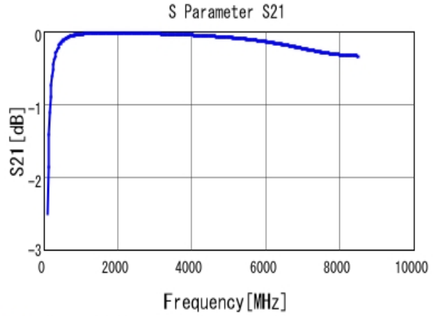
■ GRM0332C1H180GA01 S21 DCOV, 20degC
