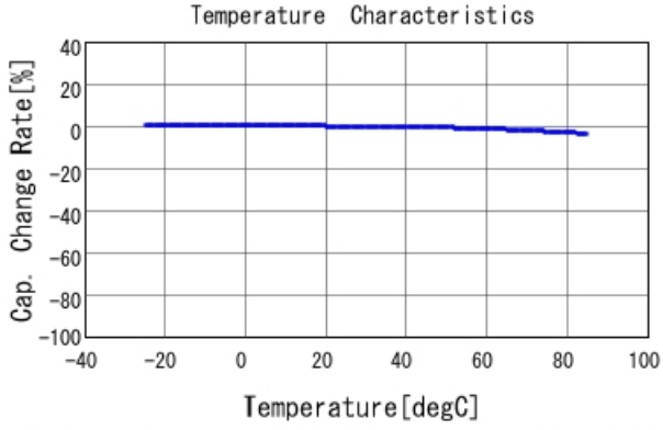
■ GRM033B31H331KA12 C-Temp. capchange, DCO. 0V, AC1. 0Vrm
