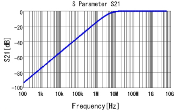
■ GRM033B31H331KA12 S21 DCOV, 20degC
