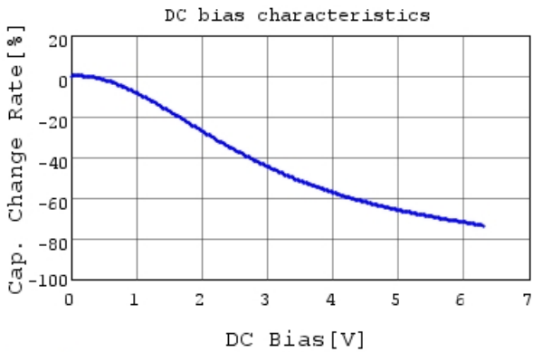
GRM022R60J223KE15 C-DC bias capchange, 25.0c
