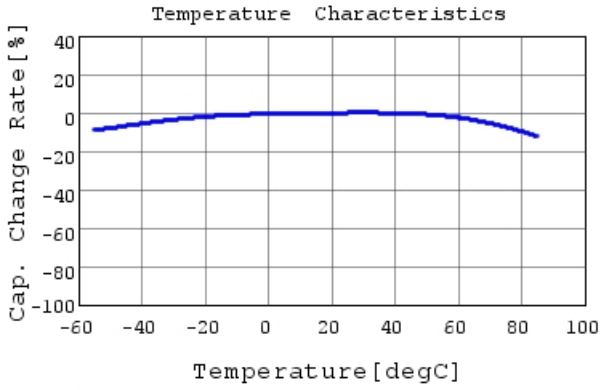
GRM022R60J223KE15 C-Temp. capchange, DC0.0V,
