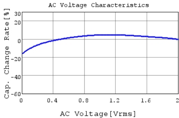
GRM022R60J223KE15 C-AC Voltage capchange, Dc
