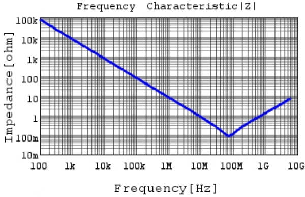
GRM022R60J223KE15 |Z| DCOV, 25degC
