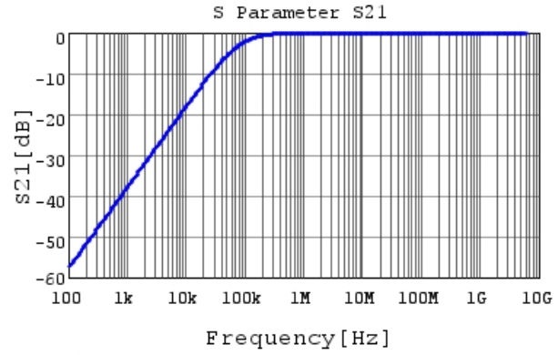
GRM022R60J223KE15 S21 DC0V,25degC
