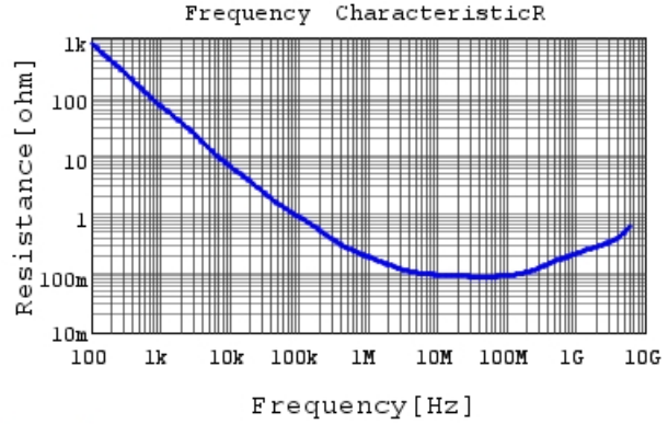
GRM022R60J223KE15 R DCOV, 25degC
