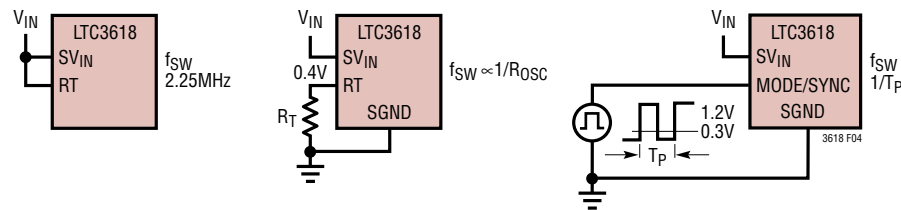
Figure 4. Setting the Switching Frequency
