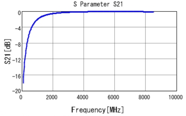
GRM0335C1E2R0BA01 S21 DCOV, 25degC
