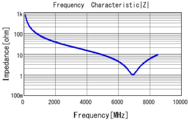
GRM0335C1E2R0BA01 |Z| DCOV, 25degC
