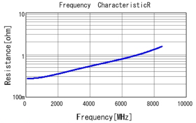
GRM0335C1E2R0BA01 R DCOV, 25degC
