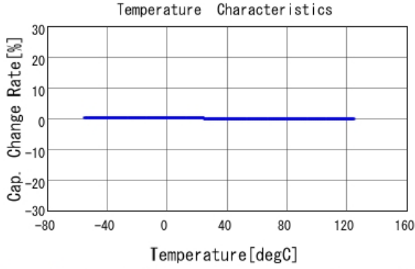
GRM0335C1E2R0BA01 C-Temp. capchange, DCOV, AC1Vrms
