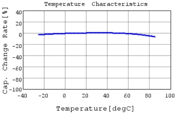
GRM033B31C104ME84 C-Temp. capchange, DC0.0V,
