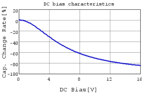
GRM033B31C104ME84 C-DC bias capchange, 20.0c
