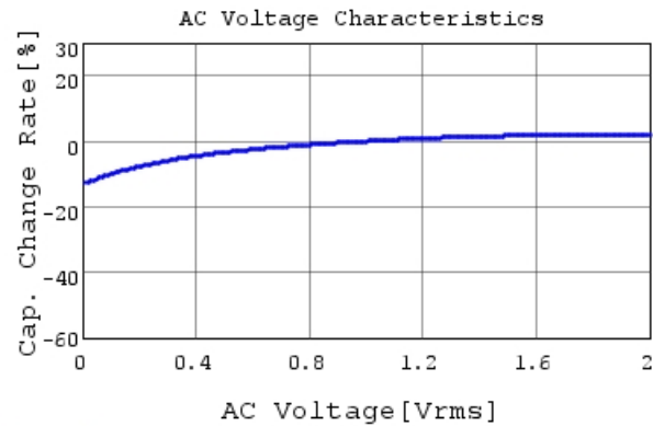
GRM033B31C104ME84 C-AC Voltage capchange, DC
