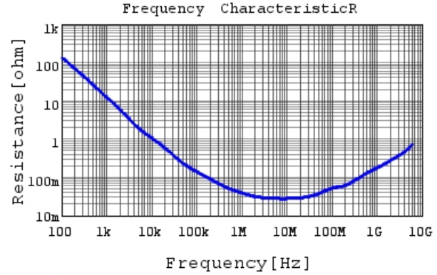
GRM033B31C104ME84 R DC0V, 20degC
