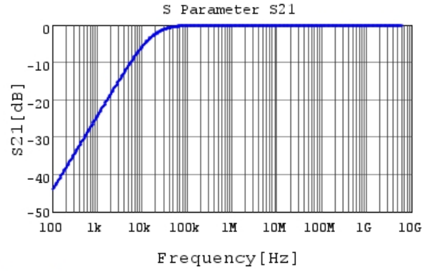
GRM033B31C104ME84 S21 DC0V,20degC
