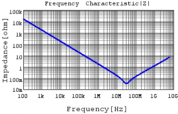
GRM033B31C104ME84 |Z| DC0V, 20degC
