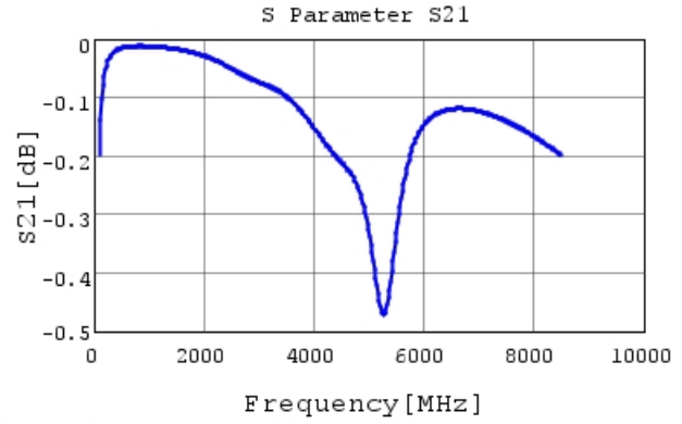
GRM0335C2A750JA01 S21 DCOV, 25degC
