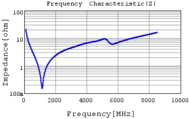
GRM0335C2A750JA01 |Z| DCOV, 25degC
