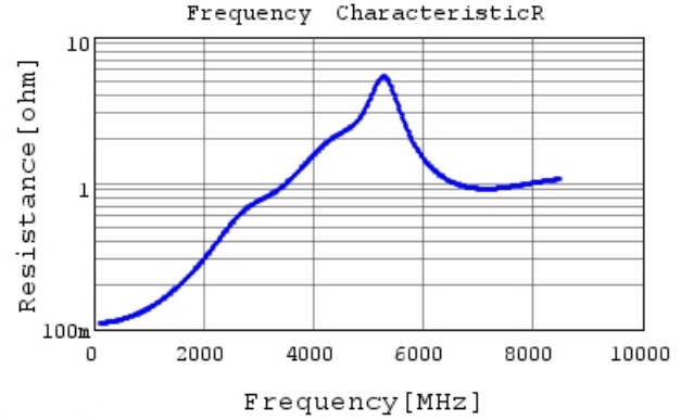
GRM0335C2A750JA01 R DCOV, 25degC
