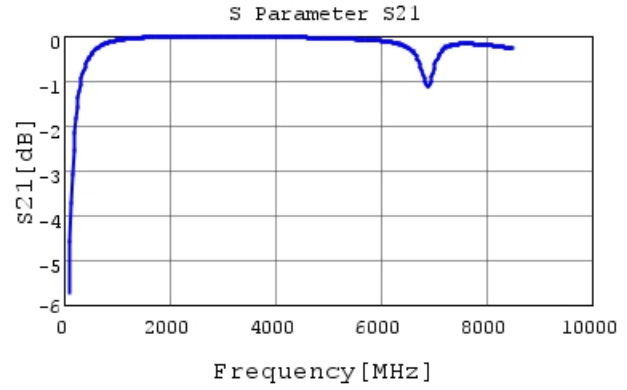
GCQ1555C1H9R6BB01 S21 DCOV, 25degC
