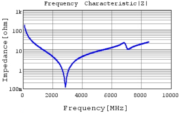
GCQ1555C1H9R6BB01 |Z| DC0V, 25degC
