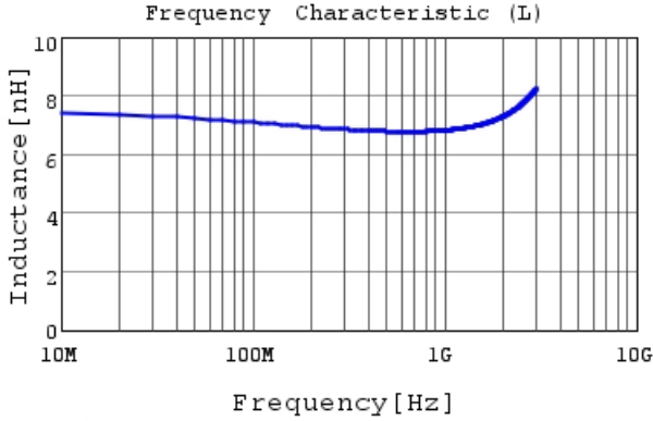
LQP03TN6N8JZ2 L
