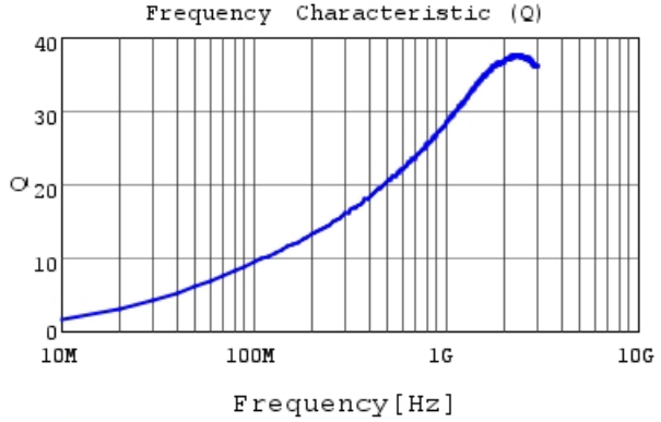
LQP03TN6N8JZ2 Q
