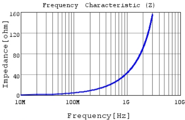
LQP03TN6N8JZ2 |Z|
