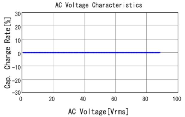
GRM21A5C2E150JW01 C-AC Voltage capchange, DCOV, 25
