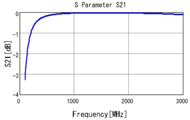
GRM21A5C2E150JW01 S21 DCOV, 25degC
