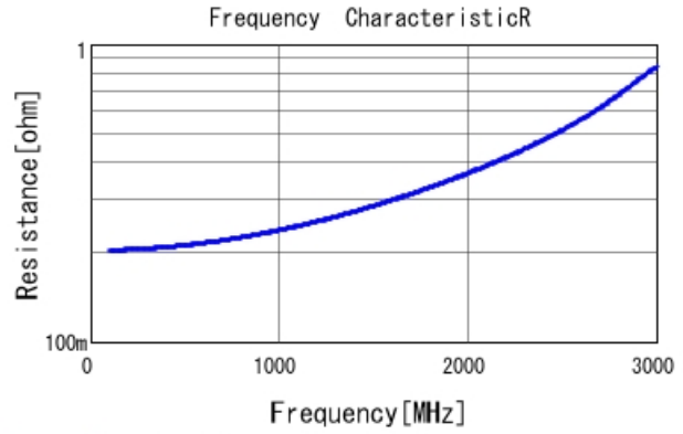
GRM21A5C2E150JW01 R DCOV, 25degC
