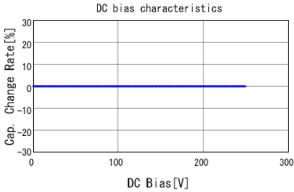
GRM21A5C2E150JW01 C-DC bias capchange, 25.0degC, A
