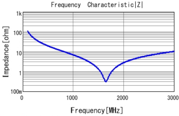
GRM21A5C2E150JW01 |Z| DCOV, 25degC
