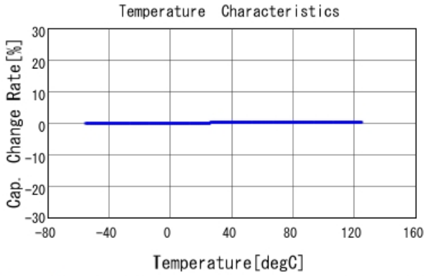
GRM21A5C2E150JW01 C-Temp. capchange, DCOV, AC1Vrms
