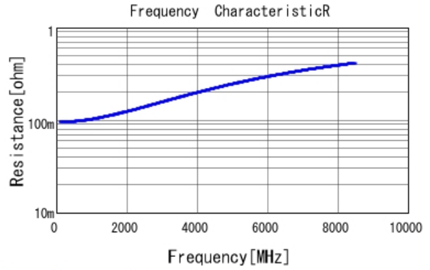
GJM0335C1E4R8BB01 R DCOV, 25degC
