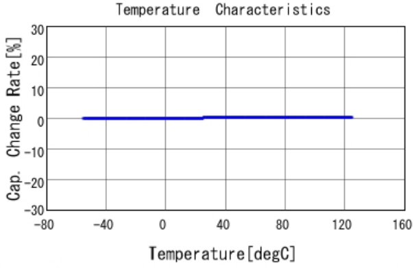
GJM0335C1E4R8BB01 C-Temp. capchange, DC0V, AC1Vrms
