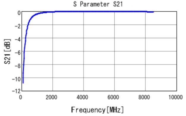
GJM0335C1E4R8BB01 S21 DC0V, 25degC
