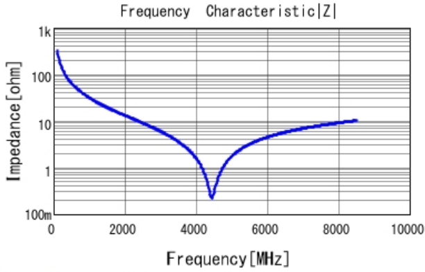
GJM0335C1E4R8BB01 |Z| DCOV, 25degC
