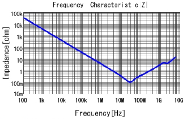
GRJ21BR71H473KE01 |Z| DCOV, 25degC
