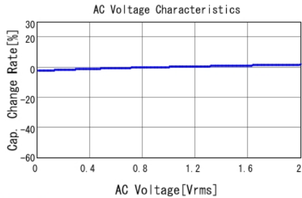
GRJ21BR71H473KE01 C-AC Voltage capchange, DCOV, 25
