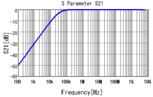
GRJ21BR71H473KE01 S21 DC0V, 25degC
