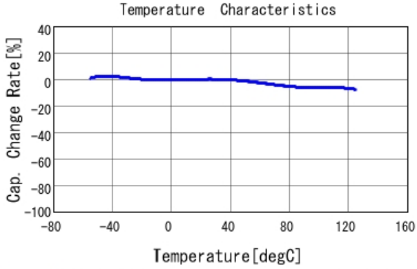
GRJ21BR71H473KE01 C-Temp. capchange, DC0.0V, AC1.C
