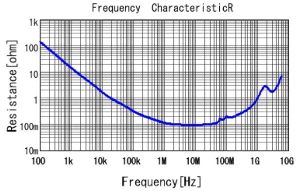
GRJ21BR71H473KE01 R DCOV, 25degC
