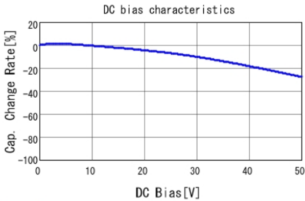
GRJ21BR71H473KE01 C-DC bias capchange, 25.0degC, A
