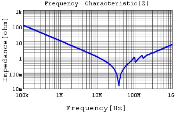
GCM32D5C2J153GX01 |Z| DC0V, 25degC
