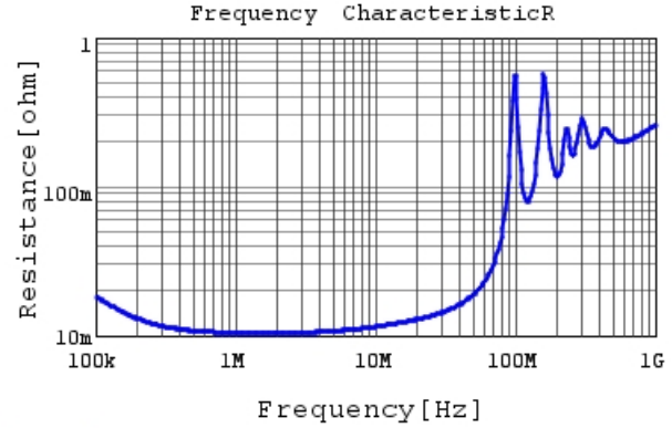
GCM32D5C2J153GX01 R DC0V, 25degC
