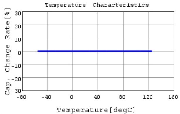
GCM32D5C2J153GX01 C-Temp. capchange, DC0V, 1
