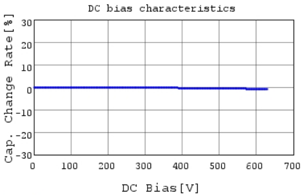
GCM32D5C2J153GX01 C-DC bias capchange, 25.0c
