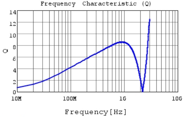
LQP02TN39NH02 Q
