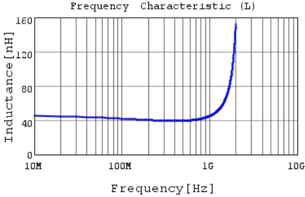
LQP02TN39NH02 L
