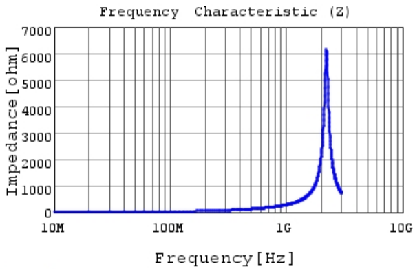
LQP02TN39NH02 |Z|
