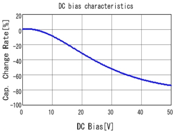
■ GRJ32ER71H106KE11 C-DC bias capchange, 25.0degC, AC1V
