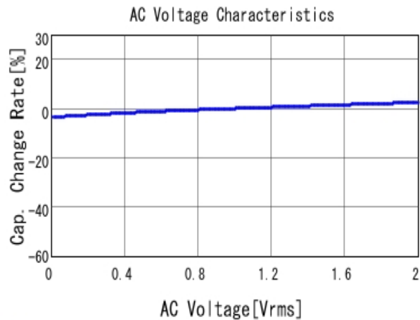
■ GRJ32ER71H106KE11 C-AC Voltage capchange, DCOV, 25.0d
