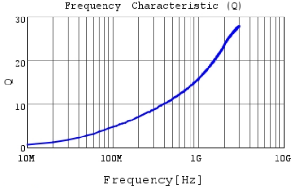
LQP02TN1N8C02 Q
