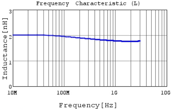
LQP02TN1N8C02 L
