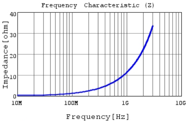
LQP02TN1N8C02 |Z|
