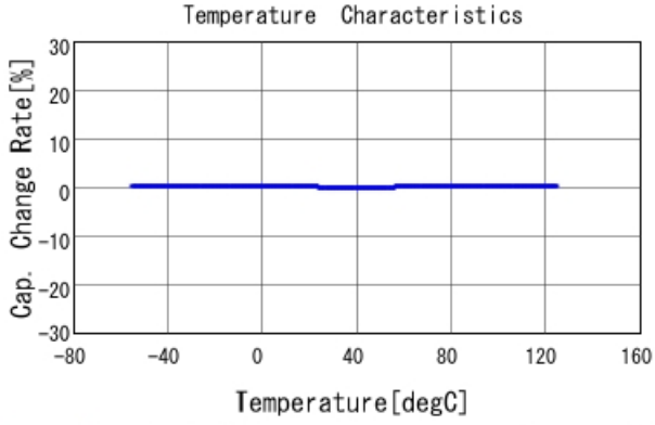
GRM1555C1HR80BA01 C-Temp. capchange, DCOV, AC1Vrms
