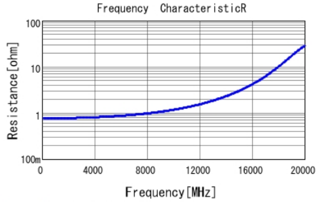
GRM1555C1HR80BA01 R DCOV, 25degC
