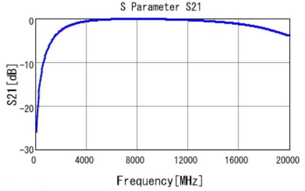
GRM1555C1HR80BA01 S21 DCOV, 25degC
