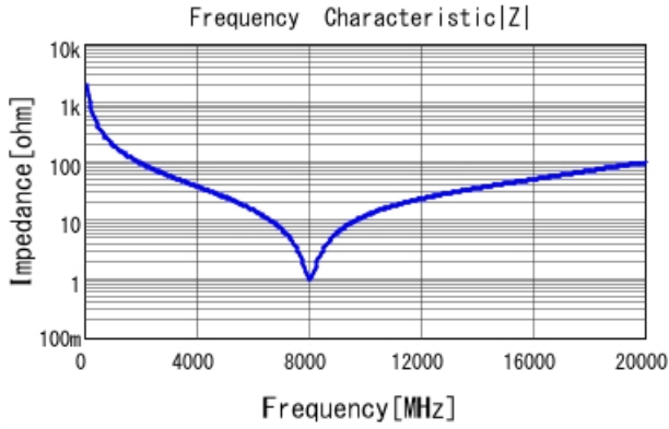
GRM1555C1HR80BA01 |Z| DCOV, 25degC
