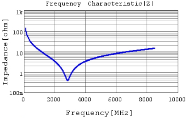
GRM0332C2A120JA01 |Z| DCOV, 20degC
