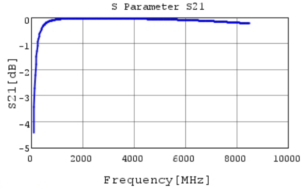
GRM0332C2A120JA01 S21 DCOV, 20degC
