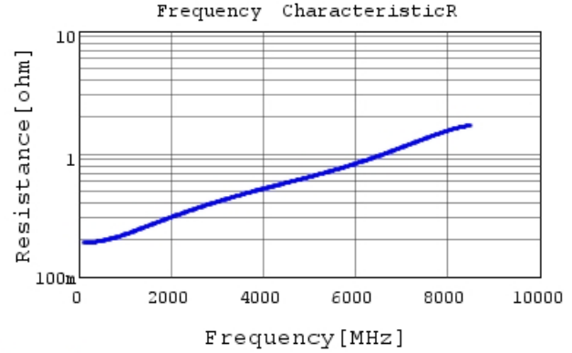
GRM0332C2A120JA01 R DCOV, 20degC
