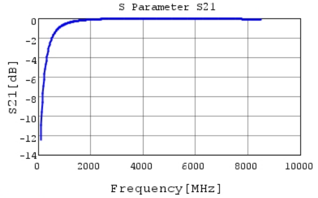
GJM0335C1E3R9CB01 S21 DCOV, 25degC
