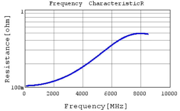
GJM0335C1E3R9CB01 R DC0V, 25degC
