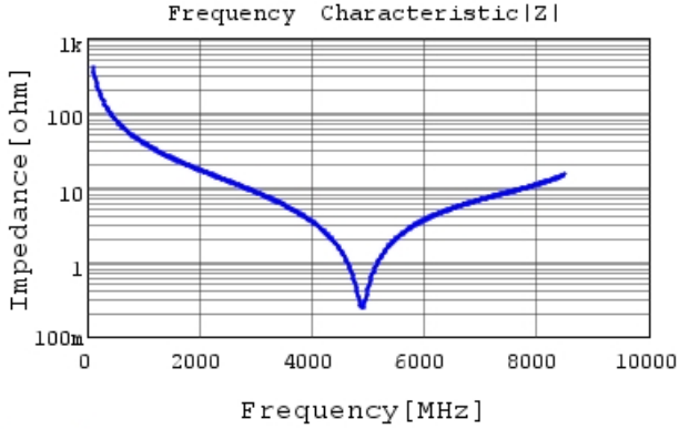
GJM0335C1E3R9CB01 |Z| DC0V, 25degC
