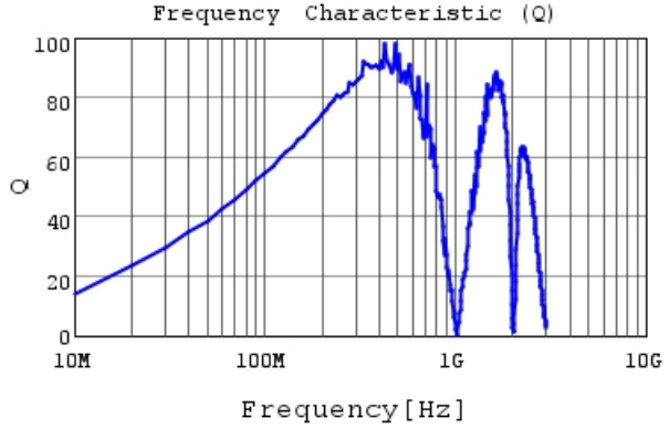
LQW2UASR15F0C Q
