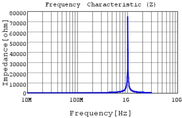
LQW2UASR15F0C |Z|
