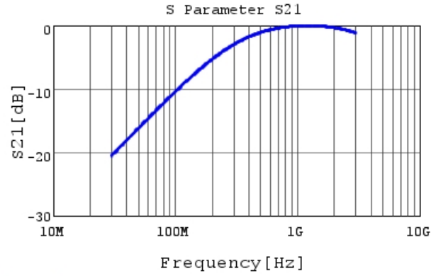
RCE5C2A5R0C0DBH03A S21 DC0V, 25degC
