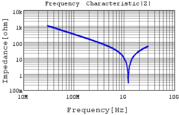
RCE5C2A5R0C0DBH03A |Z| DC0V, 25degC
