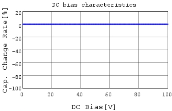
RCE5C2A5R0C0DBH03A C-DC bias capchange, 25.0
