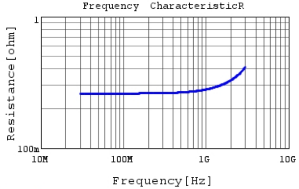
RCE5C2A5R0C0DBH03A R DC0V, 25degC
