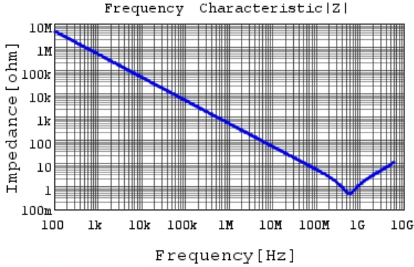
GRM033R71E331KA01 |Z| DCOV, 25degC
