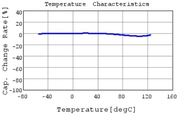
GRM033R71E331KA01 C-Temp. capchange, DC0.0V,
