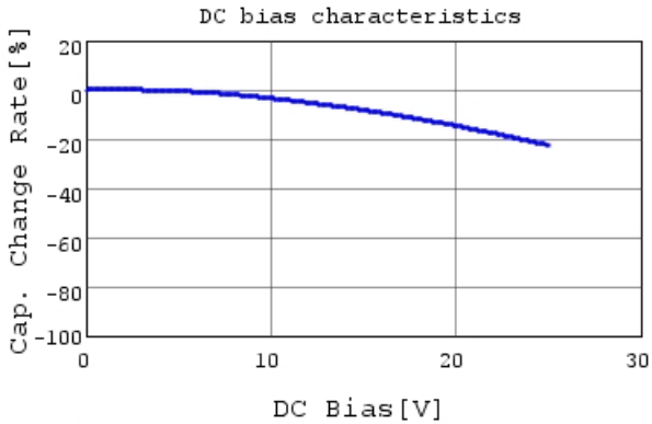
GRM033R71E331KA01 C-DC bias capchange, 25.0c
