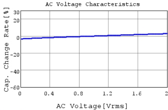
GRM033R71E331KA01 C-AC Voltage capchange, Dc
