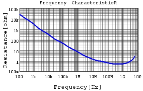
GRM033R71E331KA01 R DCOV, 25degC
