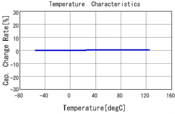
GJM0335C1E2R0BB01 C-Temp. capchange, DCOV, AC1Vrms
