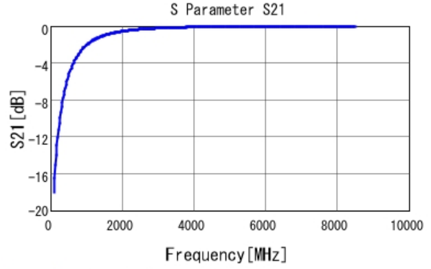
GJM0335C1E2R0BB01 S21 DCOV, 25degC
