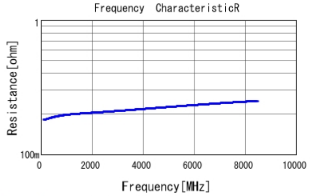
GJM0335C1E2R0BB01 R DCOV, 25degC
