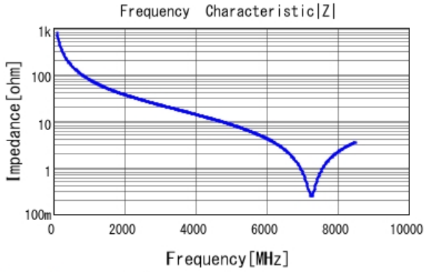
GJM0335C1E2R0BB01 |Z| DCOV, 25degC
