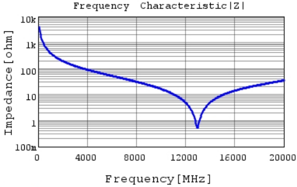
GCQ1555C1HR40BB01 |Z| DC0V, 25degC
