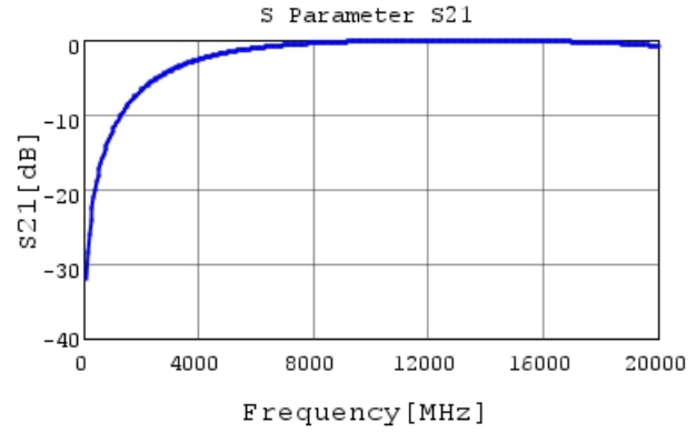
GCQ1555C1HR40BB01 S21 DCOV, 25degC
