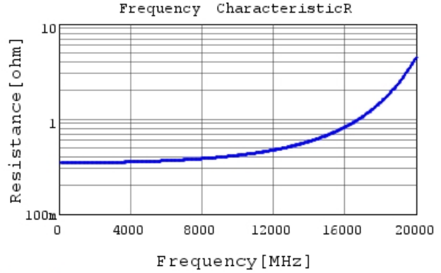
GCQ1555C1HR40BB01 R DC0V, 25degC
