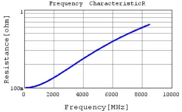
GJM0335C1E7R8CB01 R DC0V, 25degC
