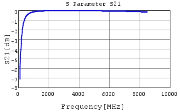
GJM0335C1E7R8CB01 S21 DCOV, 25degC
