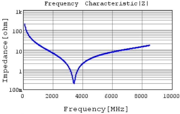
GJM0335C1E7R8CB01 |Z| DC0V, 25degC
