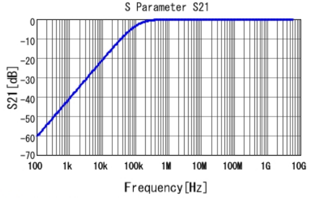
■ GRM033R61A153KE84 S21 DCOV, 25degC
