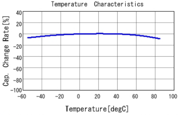
■ GRM033R61A153KE84 C-Temp. capchange, DCO. 0V, ACO. 5Vrm
