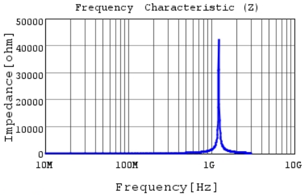
LQW2UAS82NJ0C |Z|
