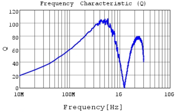
LQW2UAS82NJ0C Q
