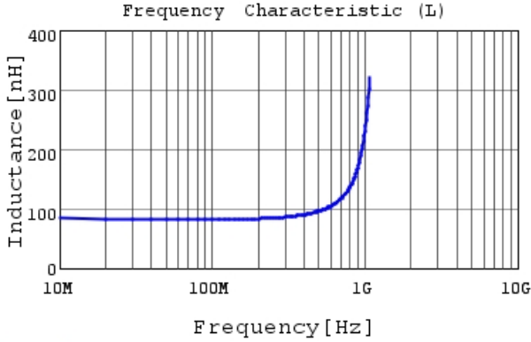
LQW2UAS82NJ0C L
