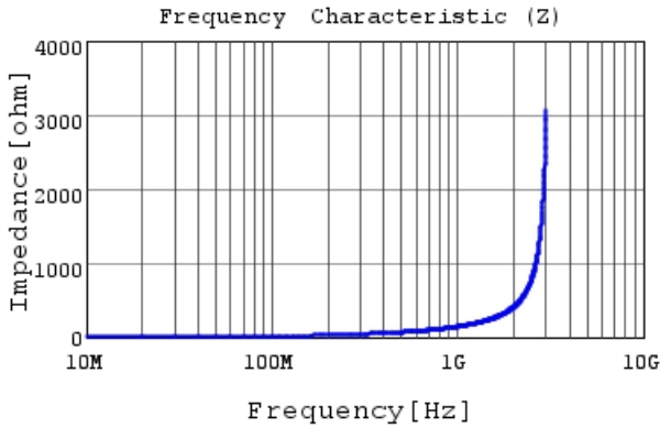
LQP02TN22NJ02 |Z|
