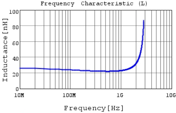
LQP02TN22NJ02 L
