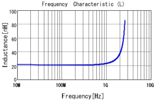
LQW2UAS22NG00 L
