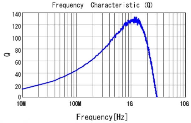
LQW2UAS22NG00 Q
