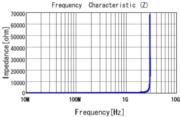
LQW2UAS22NG00 |Z|
