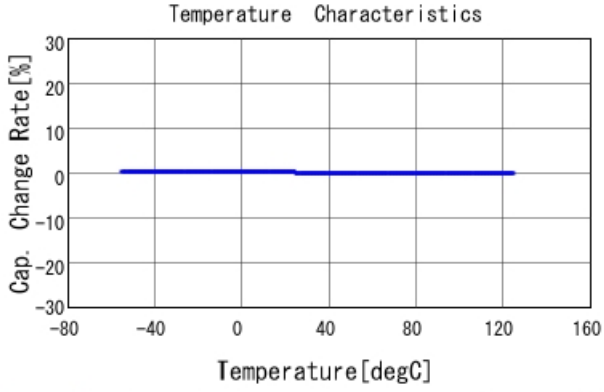
GRM1885C2A120JA01 C-Temp. capchange, DCOV, AC1Vrms
