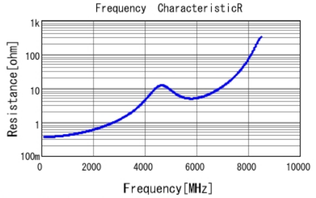
GRM1885C2A120JA01 R DCOV, 25degC
