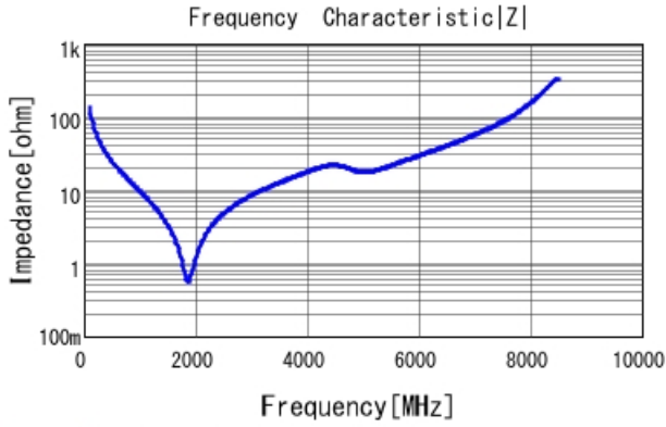
GRM1885C2A120JA01 |Z| DCOV, 25degC
