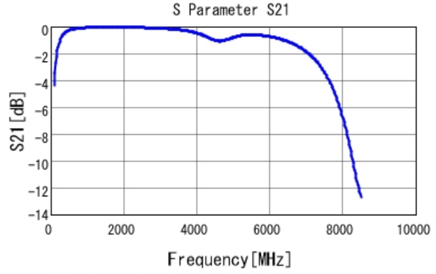
GRM1885C2A120JA01 S21 DCOV, 25degC
